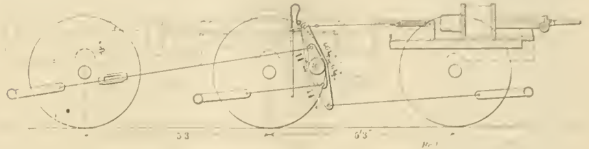
DIVIDED OR TWIN BRAKES FOR SIX WHEEL TRUCKS.
